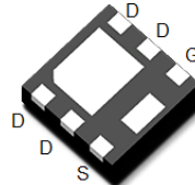
DFN2020-6L top&bottom view
