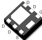
PDFN3X3-8L top&bottom view
